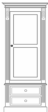
Single 2 drawer robe 80"x 29"x 23" 2034 x 730 x 585
