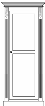
Single full hanging robe 80"x 29"x 23" 2034 x 730 x 585
