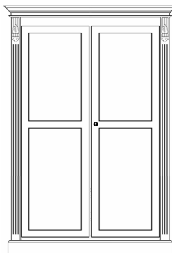
Double full hanging robe 80"x 48"x 23" 2034 x 1220 x 585
